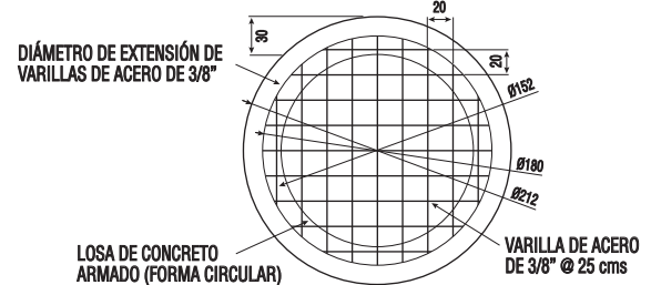
CISTERNA 2500 Lt
